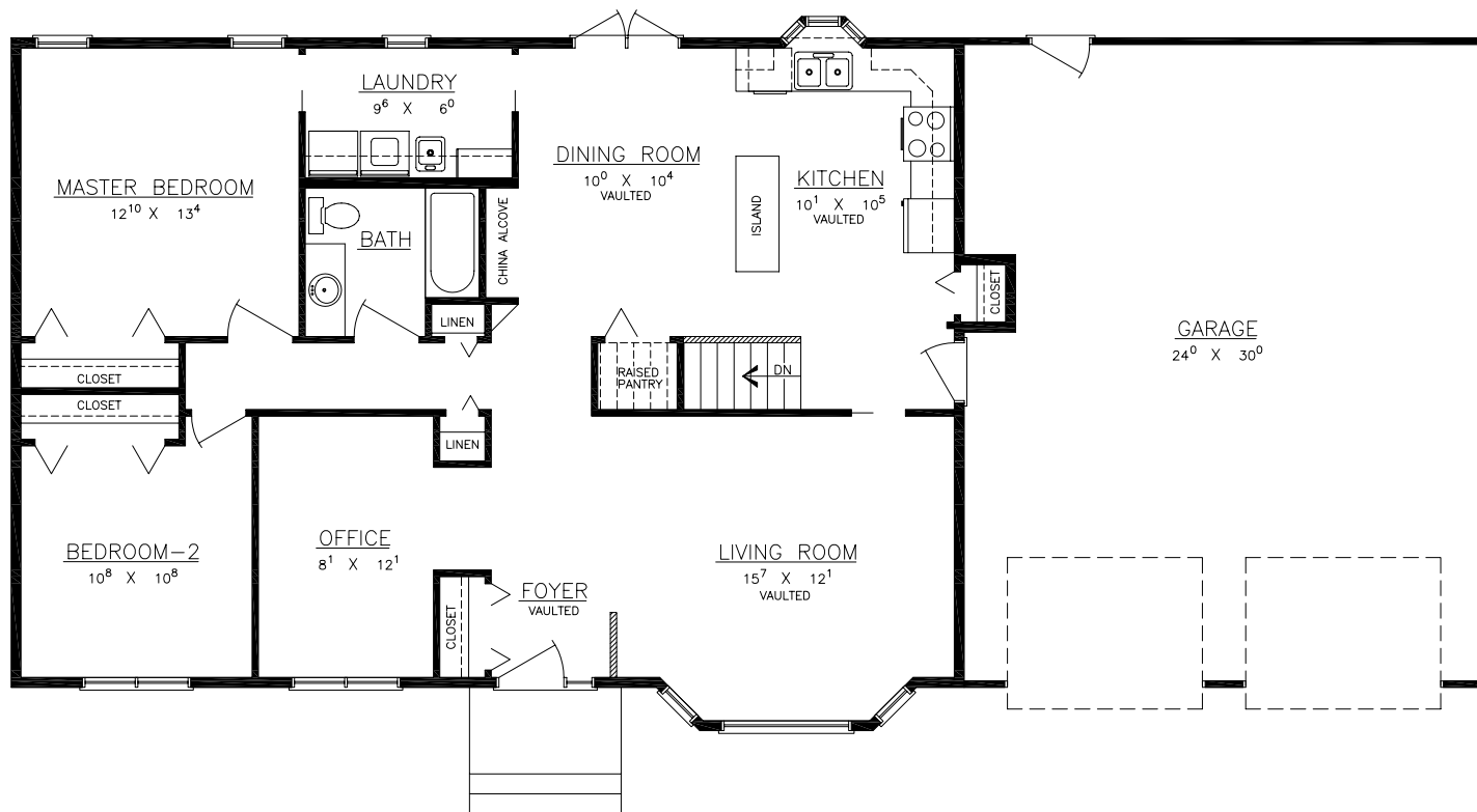
FLOOR PLAN
